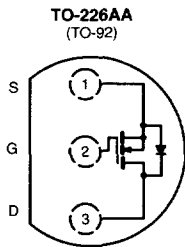
Top View VN0808L
