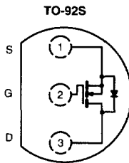
Top View VN0808LS
