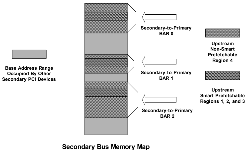
Figure 6-2. Sample Memory Map of Smart Prefetch Upstream Memory, Regions 1 through 4—Non-Transparent Mode
