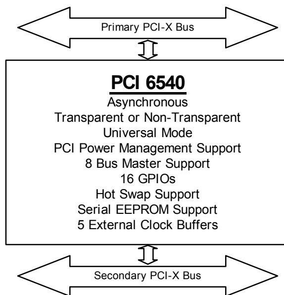
Figure 1-2. PCI 6540 PCI-X-to-PCI-X Bridge
