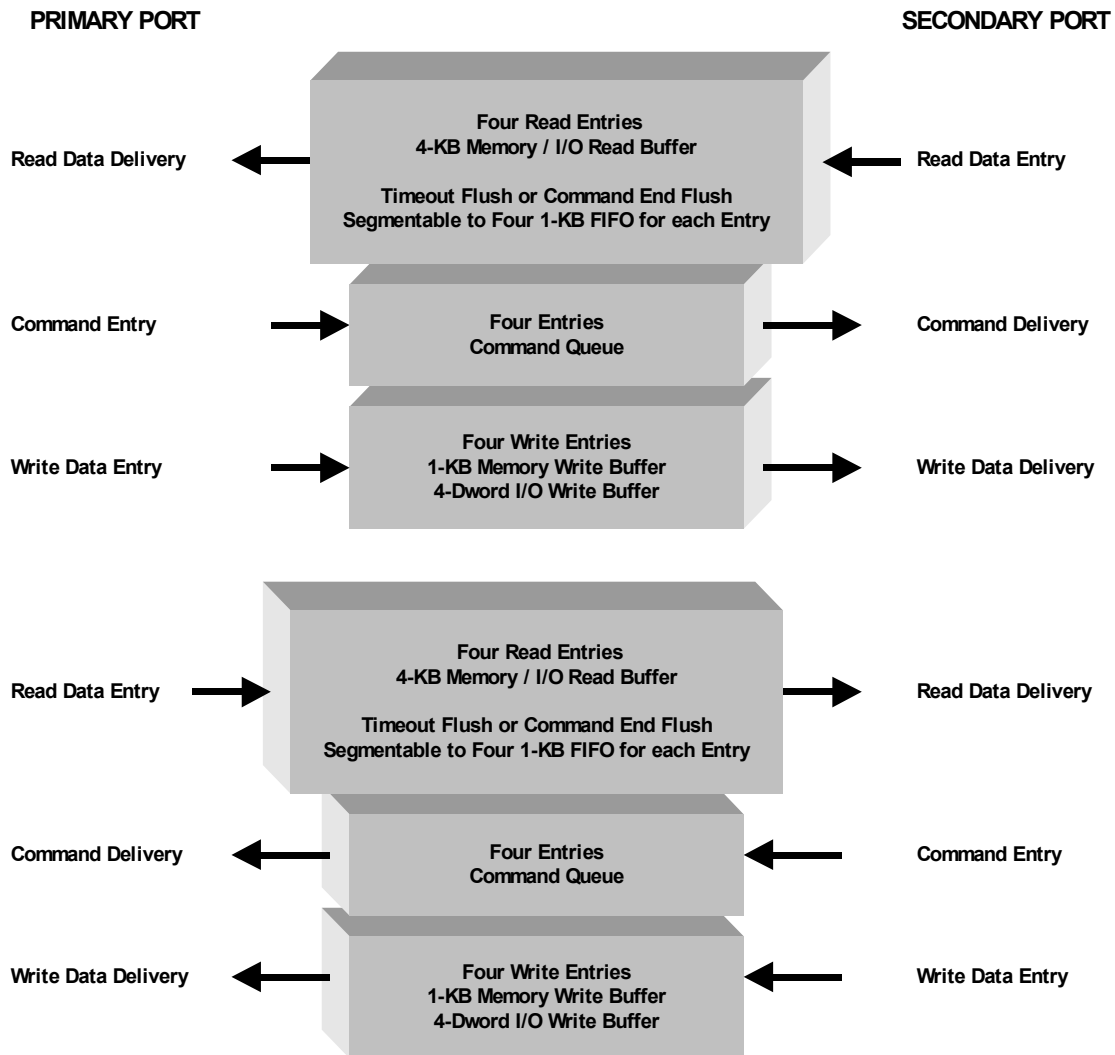
Figure 19-1. PCI 6540 FIFO Architecture
