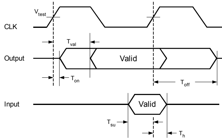
Figure 25-1. PCI/PCI-X Signal Timing Specification
