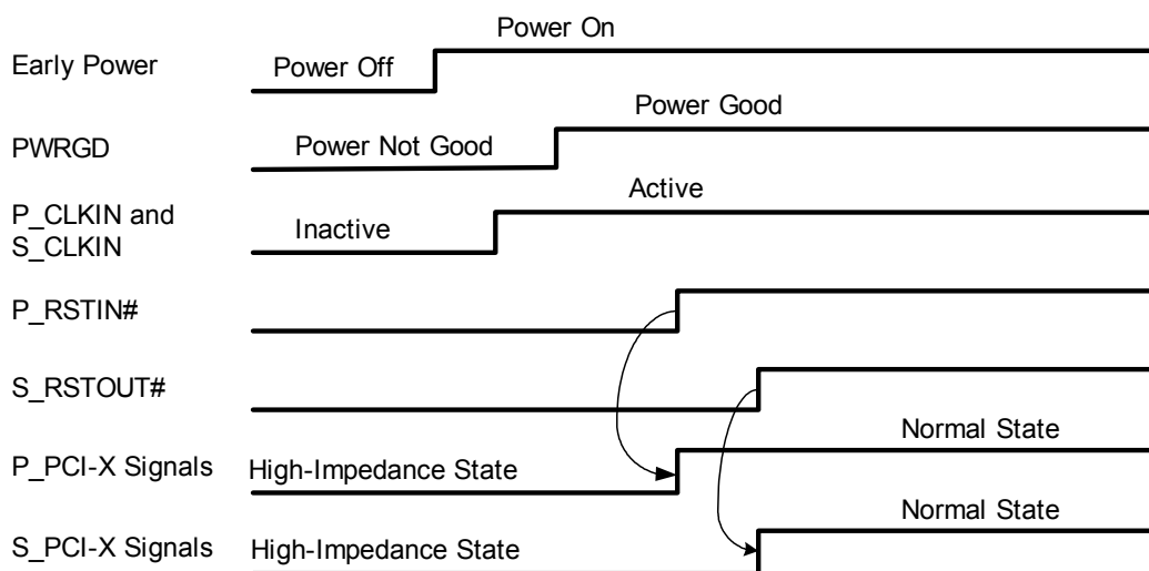
Timing Diagram 5-4. PWRGD and Resets—Universal Non-Transparent Mode
