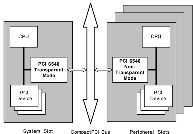
Figure 1-5. CompactPCI Universal Application
