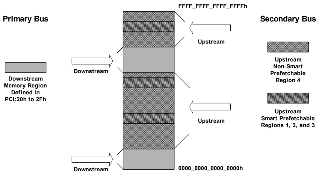
Figure 6-1. Sample Memory Map of Smart Prefetch Upstream Memory, Regions 1 through 4—Transparent Mode
