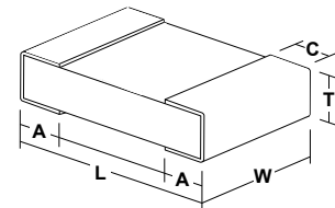
Wrap-around terminations (3 faces)
