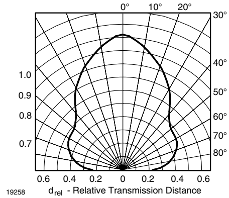
Figure 12. Horizontal Directivity
