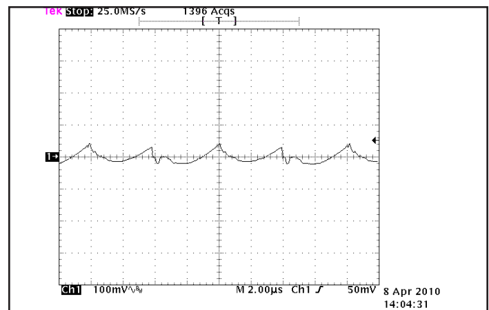
Figure 16: Output voltage ripple at nominal input voltage and rated load current (100mV/div). Load capacitance: 1\mu F ceramic capacitor and 15\mu F tantalum capacitor. Bandwidth: 20MHz. See Figure 13.
