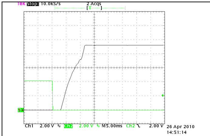
Figure 9: Turn-on transient at 50% load (resistive load) (5ms/div). Load cap: 3mF output capacitance. Input voltage pre-applied. Ch 1: Vout (2V/div), Ch 2: ON/OFF input (2V/div).
