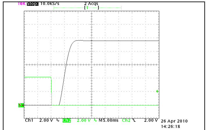
Figure 10: Turn-on transient at zero load (5ms/div). Load cap: 3mF output capacitance. Ch 1: Vout (2V/div), Ch 2: ON/OFF input (2V/div).
