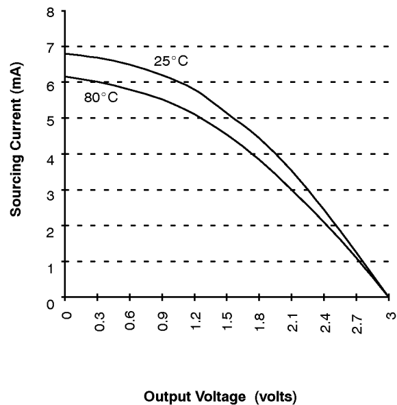
Graph 4. Digital Output Source Current DOV DD = 3.0V
