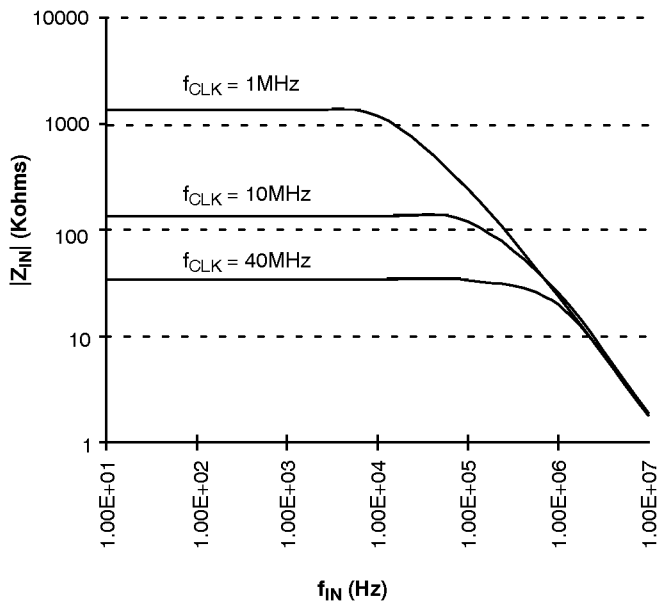
Graph 3. |Z IN | vs. f IN Log - Log Scale
