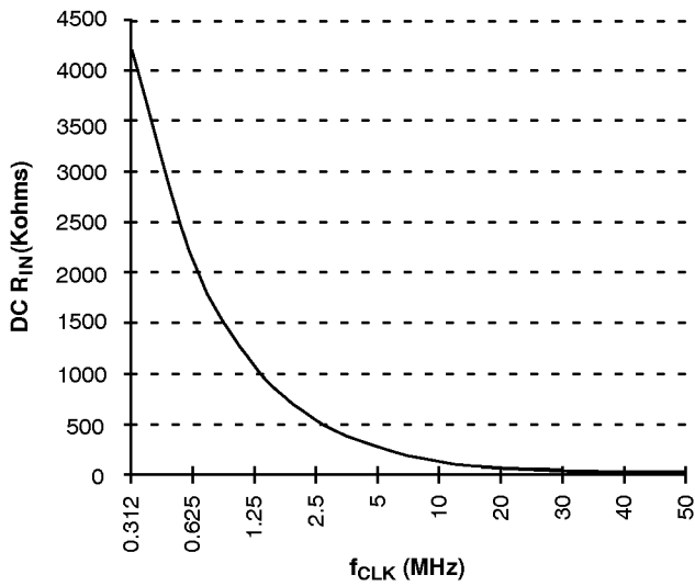
Graph 1. DC R IN vs. f CLK
