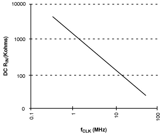
Graph 2. DC R IN vs. f CLK Log - Log Scale
