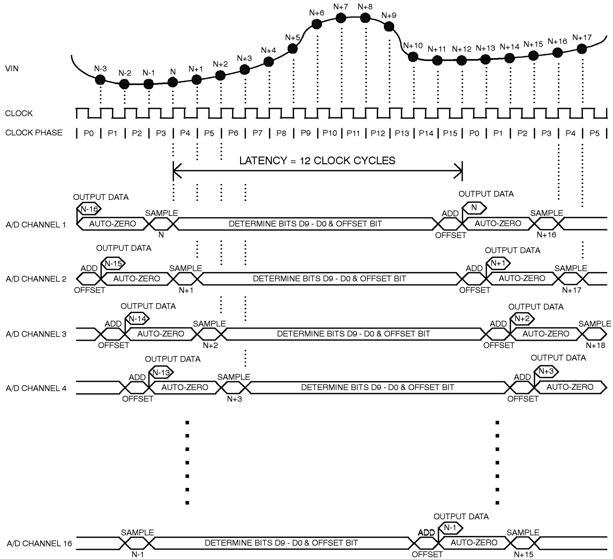
Figure 2. Timing Diagram
