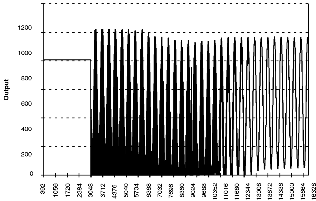
Graph 6. A/D During Initial Start-up f SAMPLE = 20MHz, f IN = 100Khz Sine Wave
