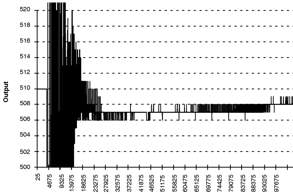
Graph 7. A/D During Initial Start-up f_{\text{SAMPLE}} = 20\text{MHz} , f_{\text{IN}} = \text{DC}
