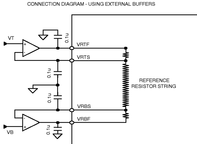
Figure 10. Circuit Diagram with External Amplifier
