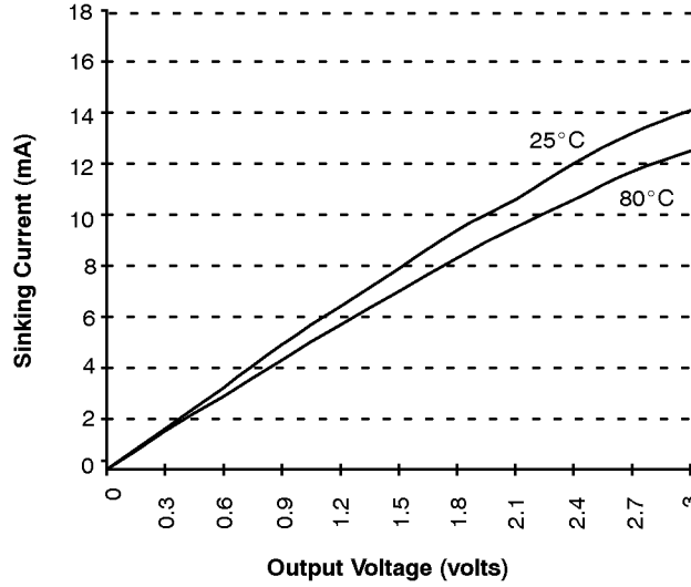
Graph 5. Digital Output Sink Current DOV DD = 3.0V
