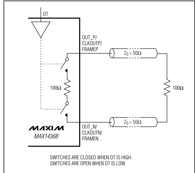
Figure 8. Double-Termination
