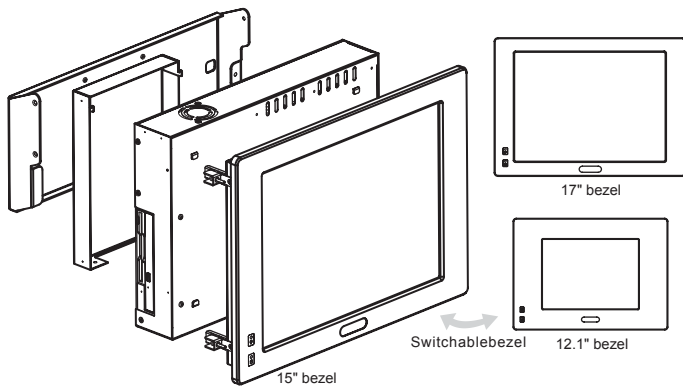
12.1" / 15" / 17" Modularizing View
