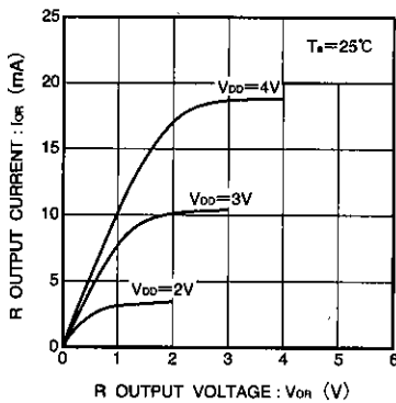
Fig. 34 IR output current vs. voltage characteristic (typical values)
