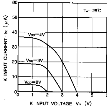
Fig. 31 IK input current vs. voltage characteristic (typical values)
