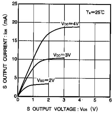
Fig. 33 IS output current vs. voltage characteristic (typical values)
