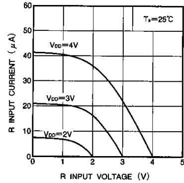
Fig. 32 IR input current vs. voltage characteristic (typical values)
