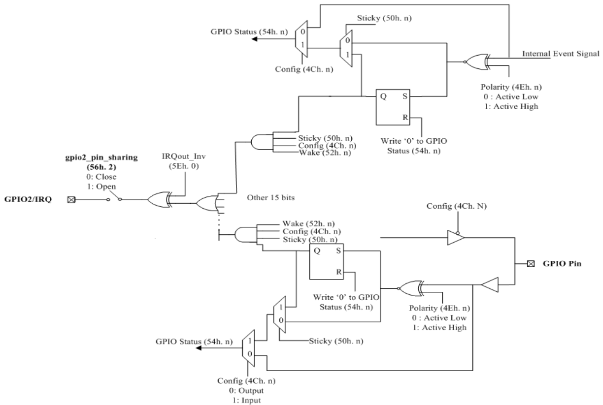
Figure 14. GPIO Implementation
