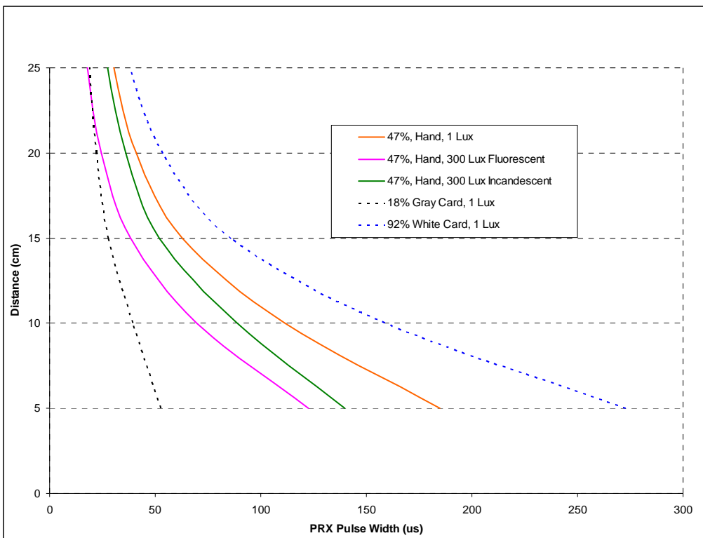
Figure 6. PRX50 Mode 2
