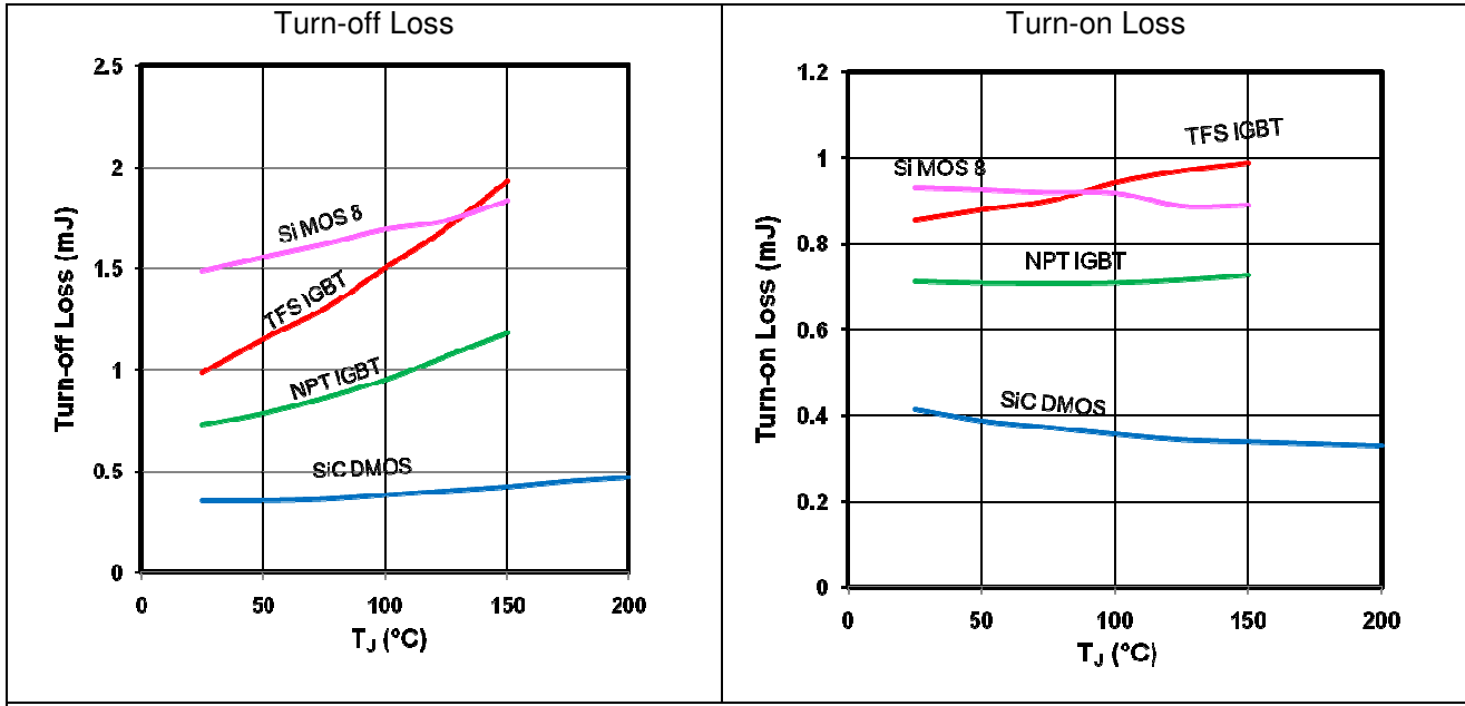
Figure 6: Switching loss vs. temperature comparison ( V_{DD} = V_{CC} = 800V , I_D = I_C = 20A , R_G = 10\Omega )
