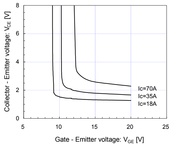
[ Inverter ] Collector-Emmitter voltage vs. Gate-Emmitter voltage (typ.) T_j = 25^\circ\text{C} / \text{chip}
