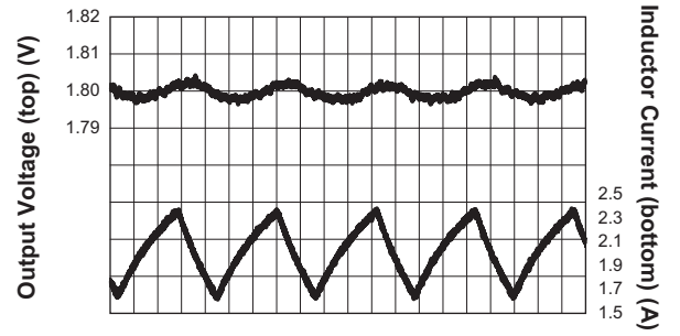
Output Ripple
