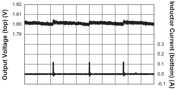
Output Ripple
