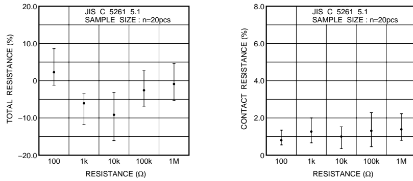
Fig.3 DC resistance : Total and contact
