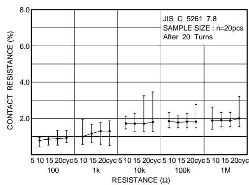
Fig.5-2 Endurance (wiper)
