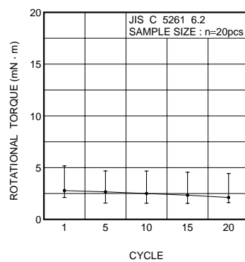
Fig.6 Rotational torque
