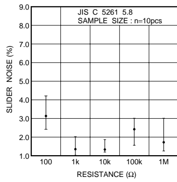
Fig.13 Wiper noise
