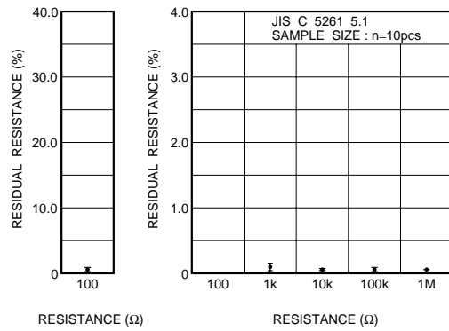
Fig.4 Residual resistance
