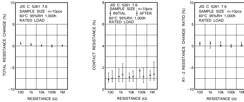
Fig.11 Endurance (under load in damp environment)
