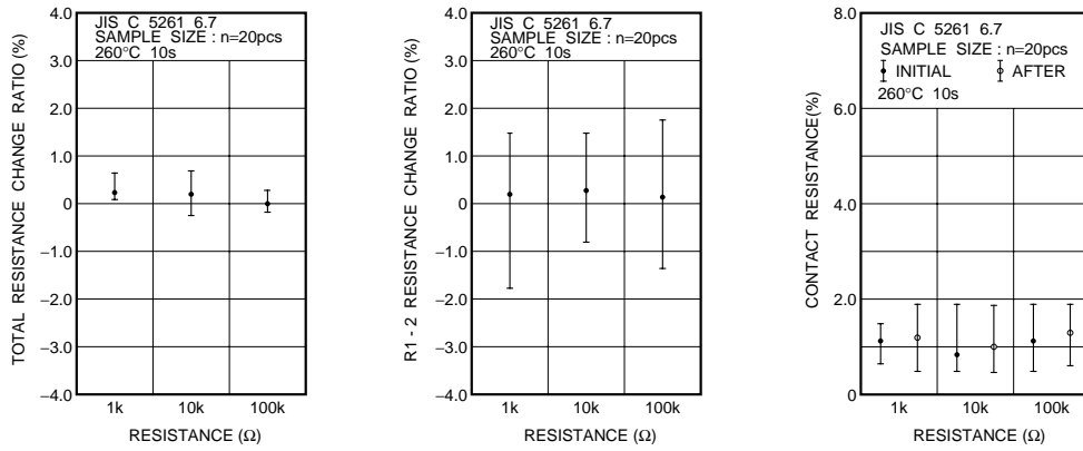
Fig.7 Resistance to soldering heat
