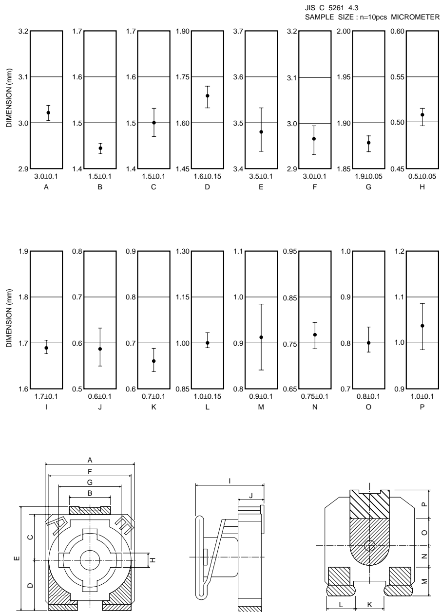
Fig.2 Dimensions
