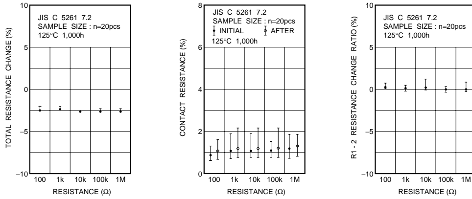
Fig.8 Resistance to dry heat
