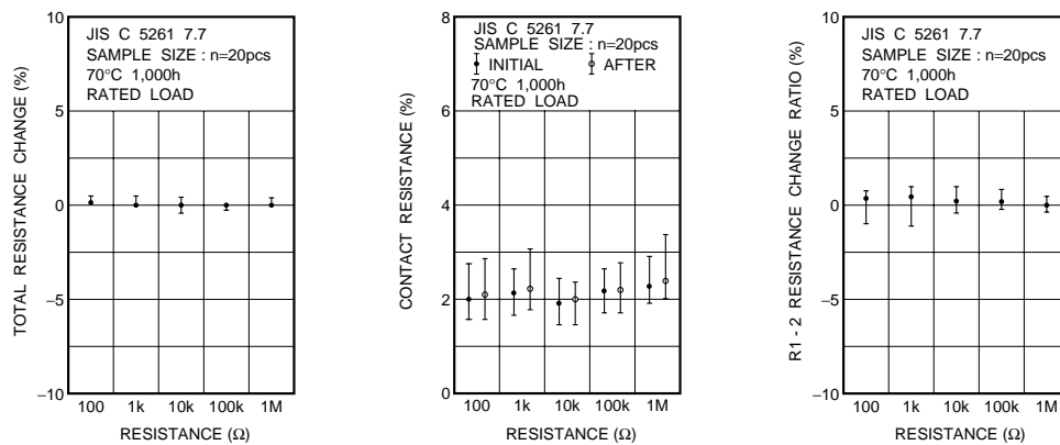
Fig.12 Endurance (rated load)
