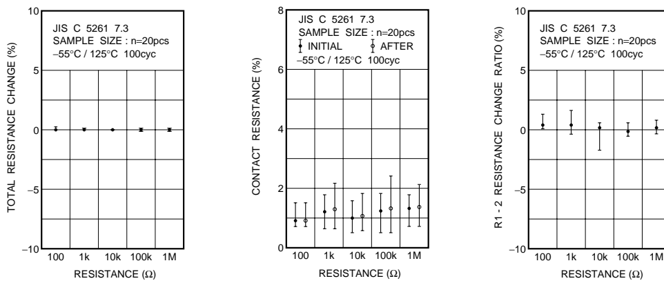
Fig.9 Temperature cycling
