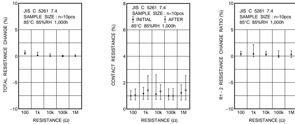
Fig.10 Resistance to humidity (steady state)
