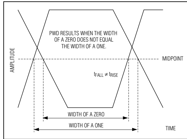
Figure 11. Pulse-Width Distortion
