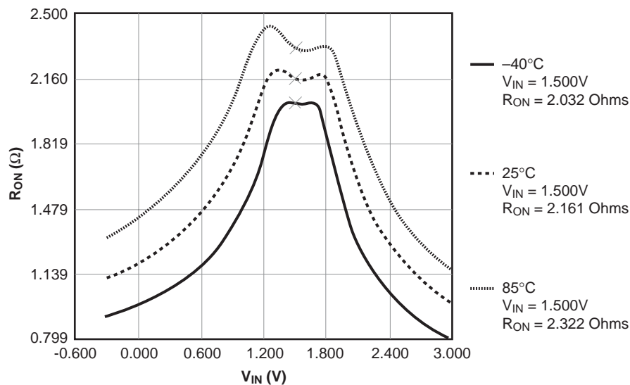
Figure 4. R_{ON} Switch On Resistance, I_{ON} = 100\text{mA} , V_{CC} = 2.7\text{V}
