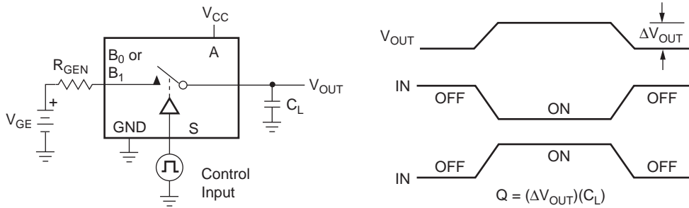
Figure 9. Charge Injection
