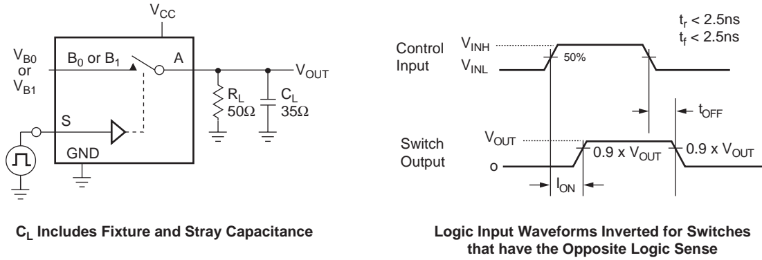
Figure 6. Turn-ON/OFF Timing
