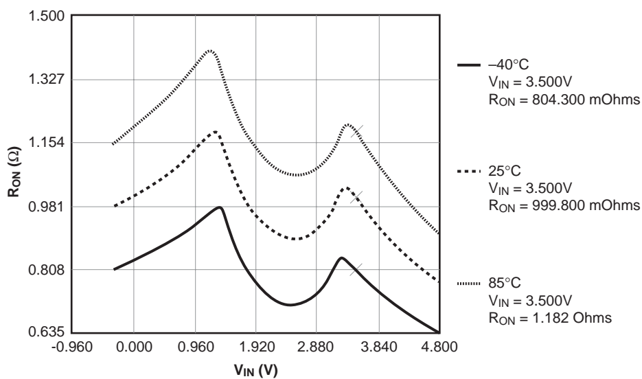
Figure 5. R_{ON} Switch On Resistance, I_{ON} = 100\text{mA} , V_{CC} = 4.5\text{V}
