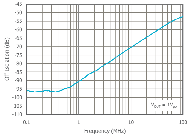
Off Isolation vs. Frequency at V_S=5\text{V}
