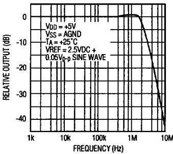
REFERENCE VOLTAGE INPUT FREQUENCY RESPONSE
