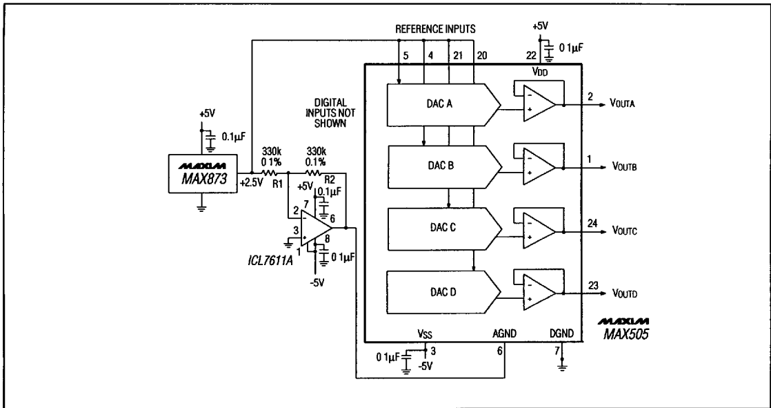
Figure 9a. MAX505 AGND Bias Circuit (Negative Offset)
