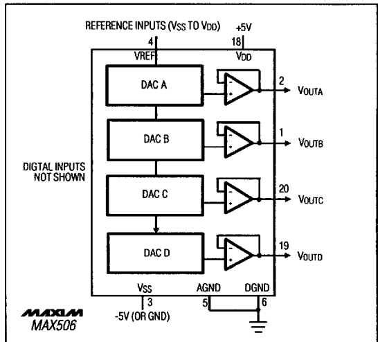
Figure 7. MAX506 Unipolar Output Circuit
