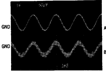
REFERENCE FEEDTHROUGH AT 400Hz
