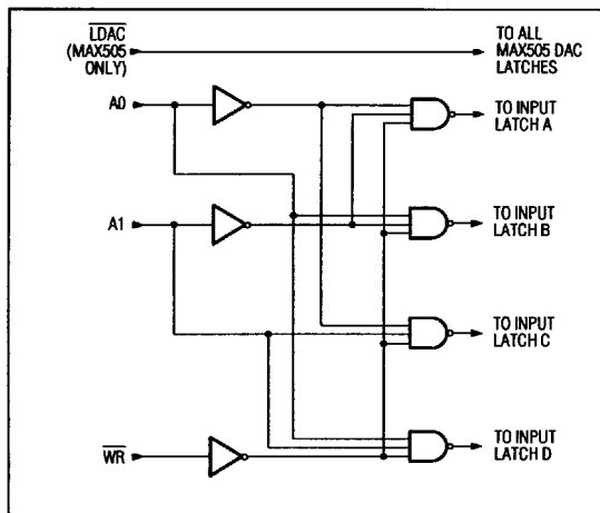
Figure 2. MAX505/MAX506 Input Control Logic
