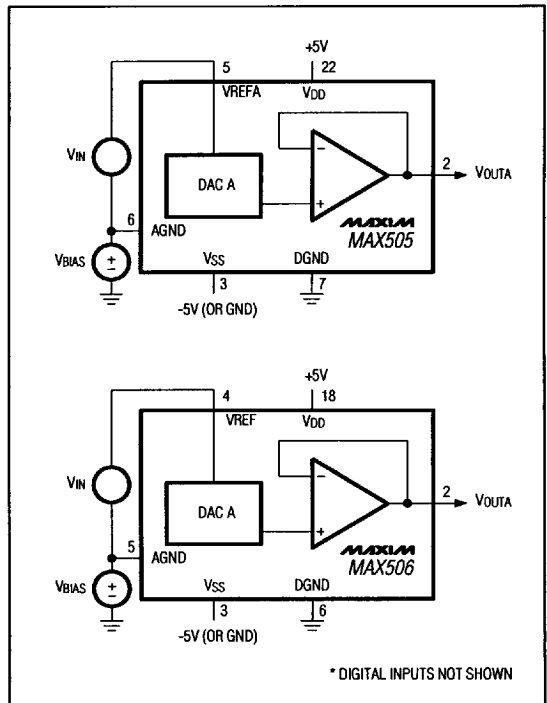
Figure 8. AGND Bias Circuits (Positive Offset)
