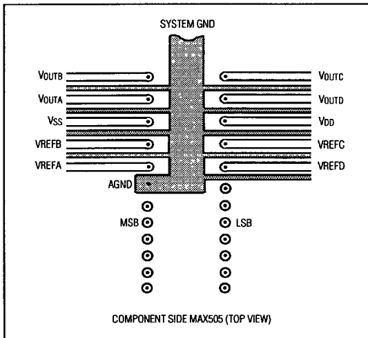
Figure 4. Suggested MAX505 PCB Layout for Minimizing Crosstalk
