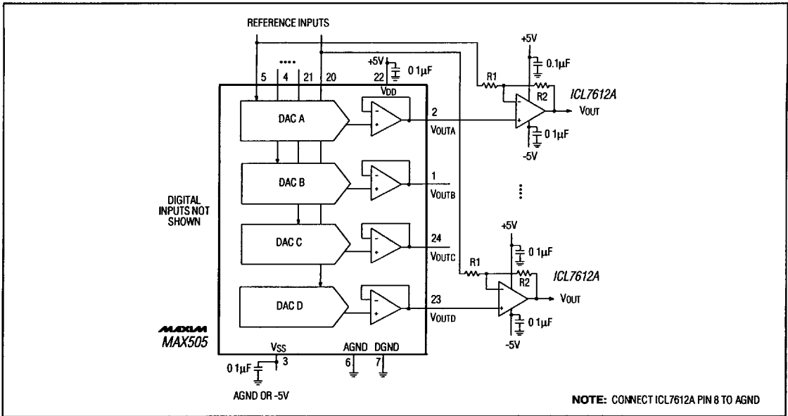
Figure 10a. MAX505 Bipolar Output Circuit
