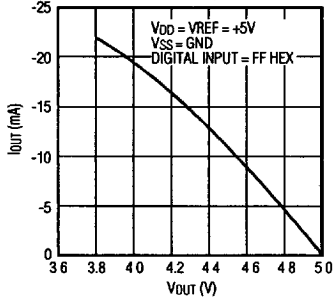
OUTPUT SOURCE CURRENT vs. V_{OUT}
