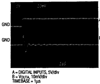
DIGITAL FEEDTHROUGH - GLITCH IMPULSE (0 TO 1 DIGITAL TRANSITION)
