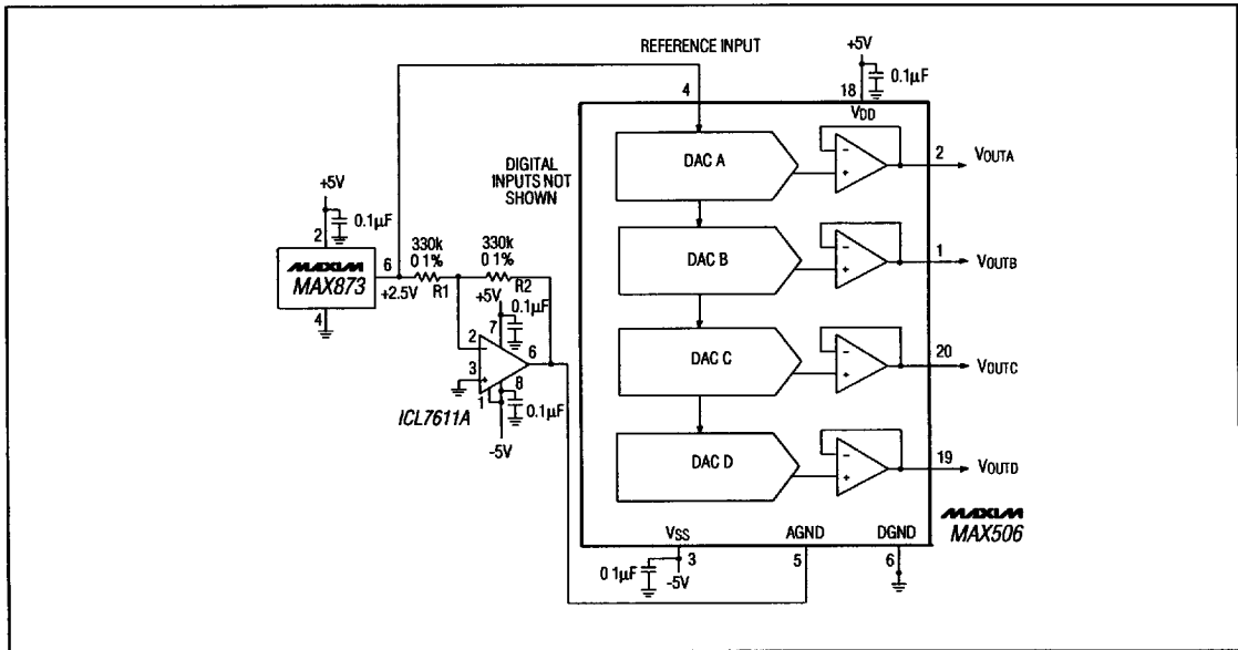
Figure 9b. MAX506 AGND Bias Circuit (Negative Offset)
