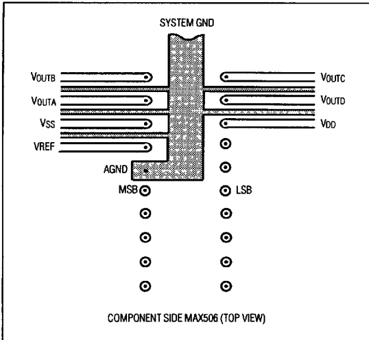
Figure 5. Suggested MAX506 PCB Layout for Minimizing Crosstalk
