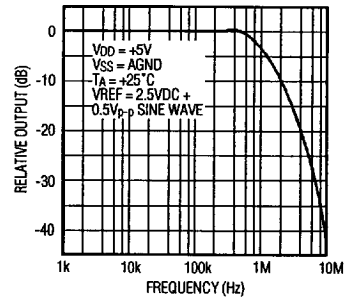
REFERENCE VOLTAGE INPUT FREQUENCY RESPONSE
