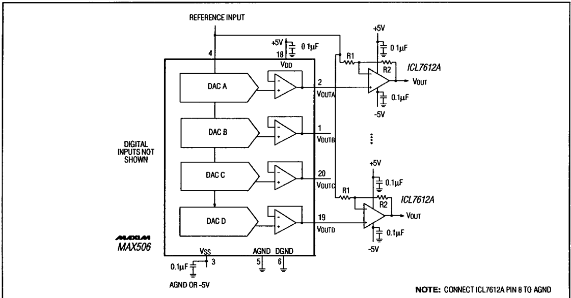
Figure 10b. MAX506 Bipolar Output Circuit
