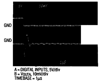
DIGITAL FEEDTHROUGH - GLITCH IMPULSE (1 TO 0 DIGITAL TRANSITION)
