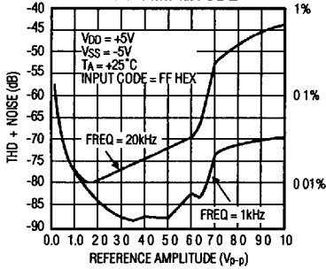
THD + NOISE AT DAC OUTPUT vs. REFERENCE FREQUENCY AND AMPLITUDE
