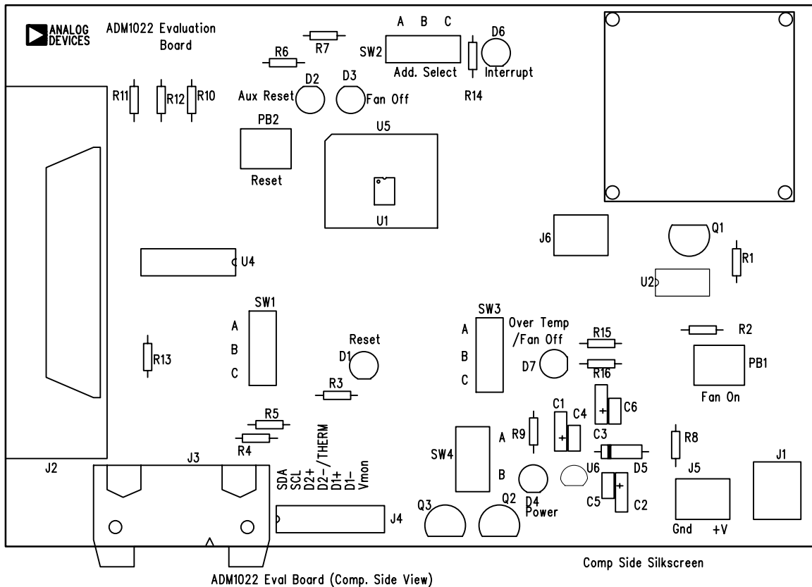
Figure 2. ADM1022 Evaluation Board SilkScreen
