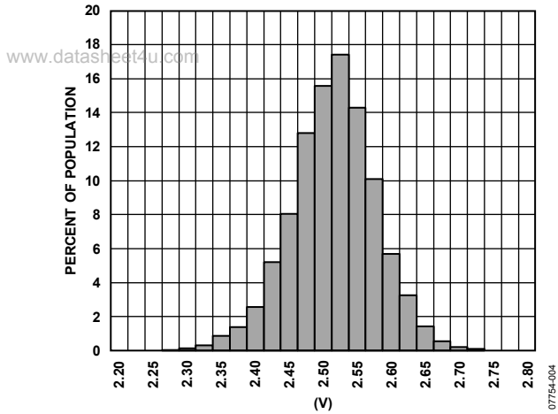
Figure 4. Null Output at 25°C ( V_{RATIO} = 5 V )
