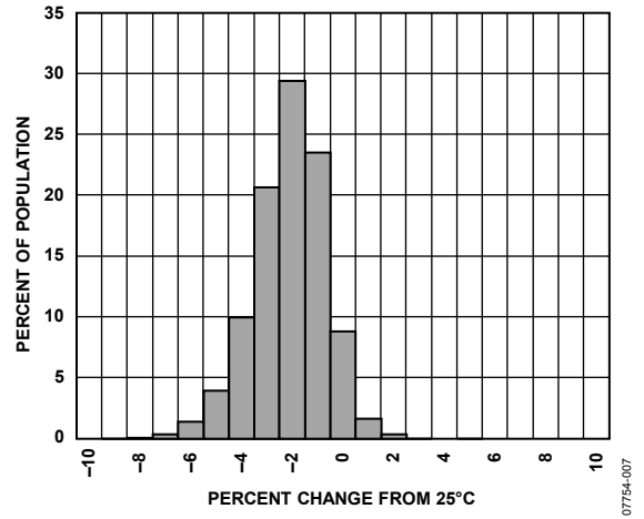
Figure 7. Sensitivity Drift over Temperature
