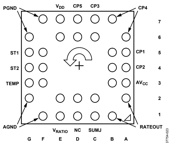
Figure 3. Pin Configuration
