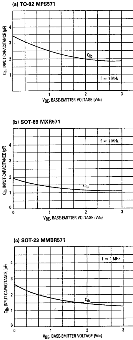
Figure 3. Input Capacitance versus Emitter Base Voltage
