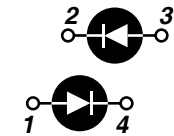
Anti-Parallel APT2X30DQ60J
