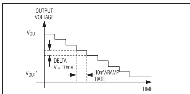
Figure 7. Ramp-Down Function
