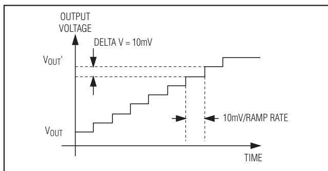
Figure 6. Ramp-Up Function
