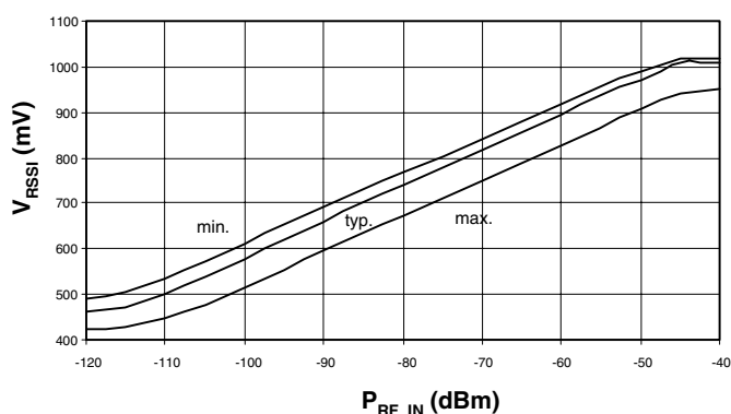
Figure 7-8. Typical RSSI Characteristic at 433.92 MHz versus Temperature and Supply Voltage
