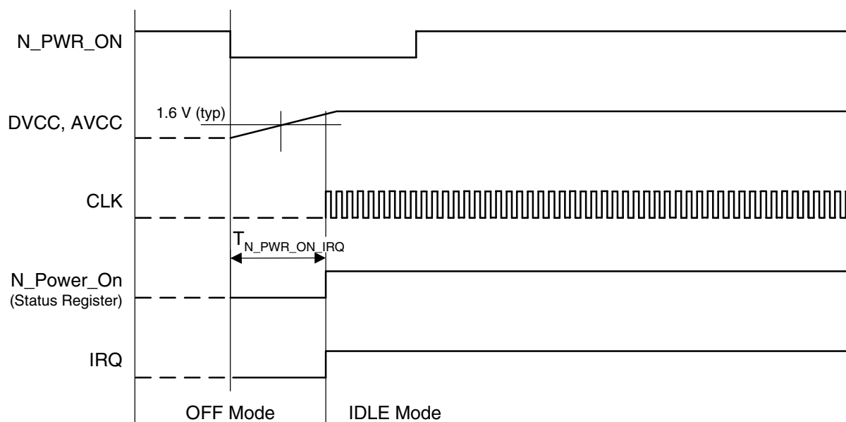
Figure 12-2. Timing Pin N_PWR_ON, Status Bit N_Power_On
