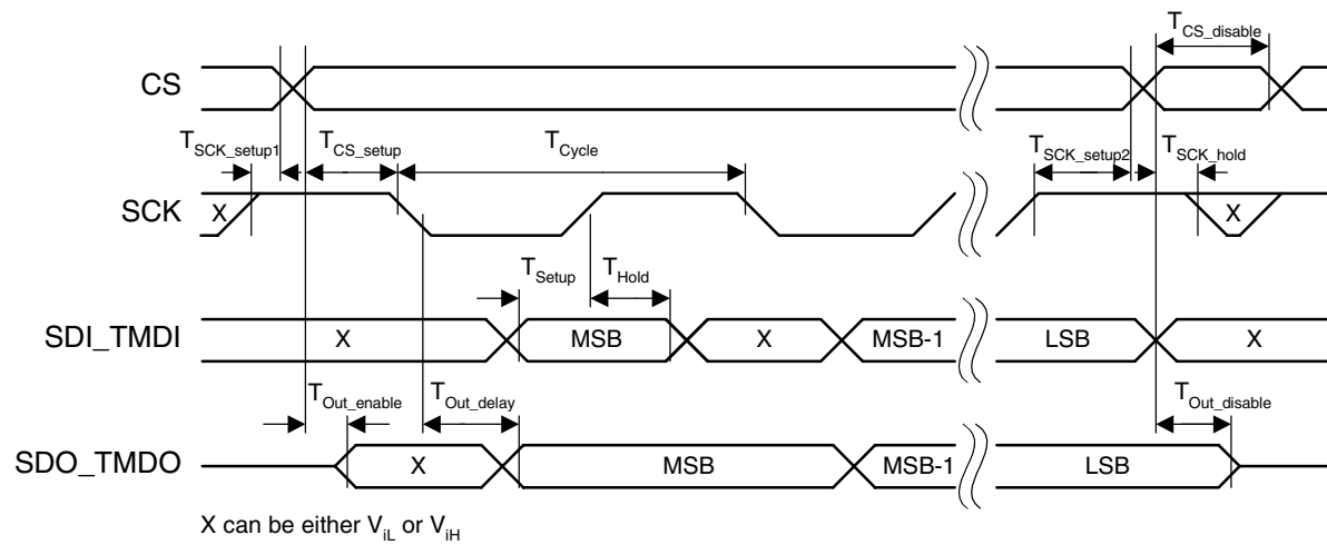
Figure 13-10. Serial Timing SCK_POL = 1, SCK_PHA = 1
