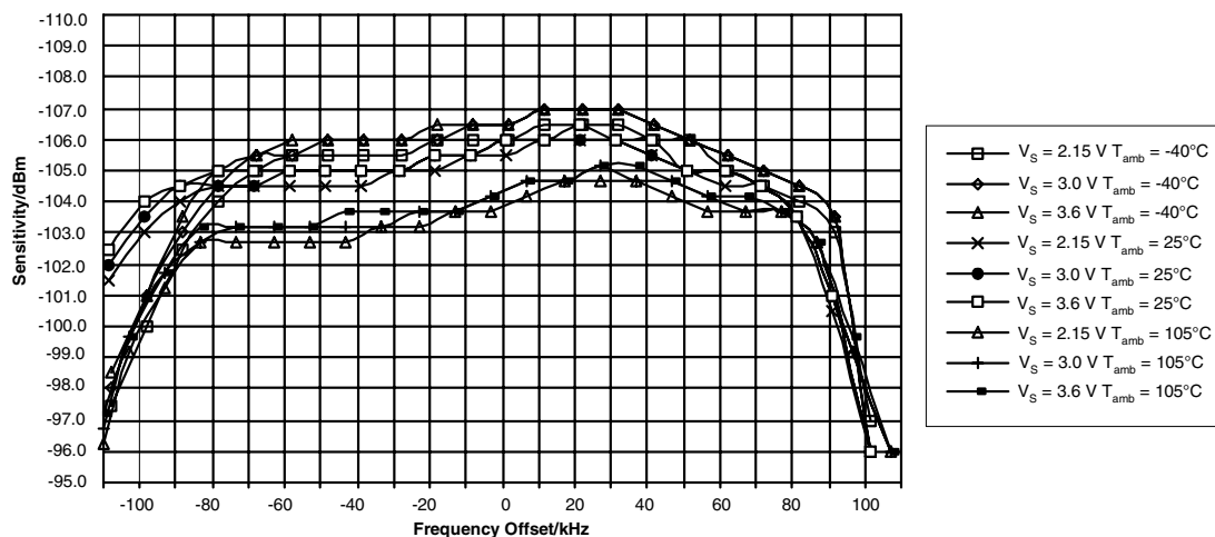
Figure 7-2. Measured Sensitivity 433.92 MHz/FSK/20 kBaud/±19.5 kHz/Manchester versus Frequency Offset, Temperature and Supply Voltage
