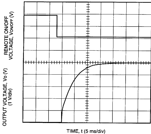
Figure 13. Typical Start-Up from Remote On/Off JC100A1; I_o = \text{Full Load}
