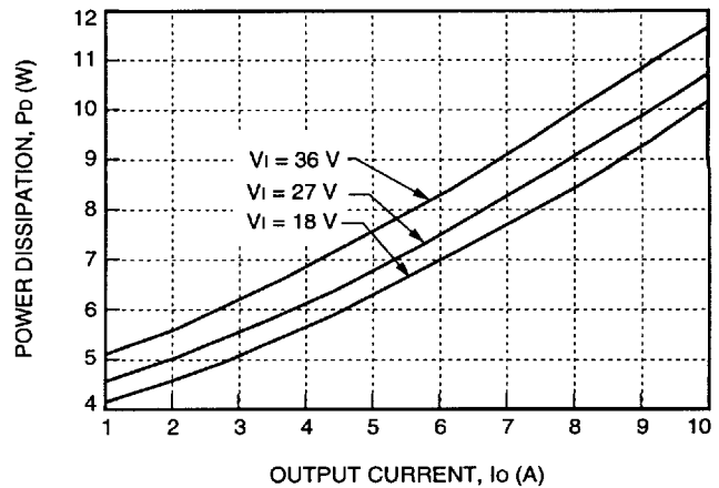
Figure 25. JC050A Power Dissipation vs. Output Current
