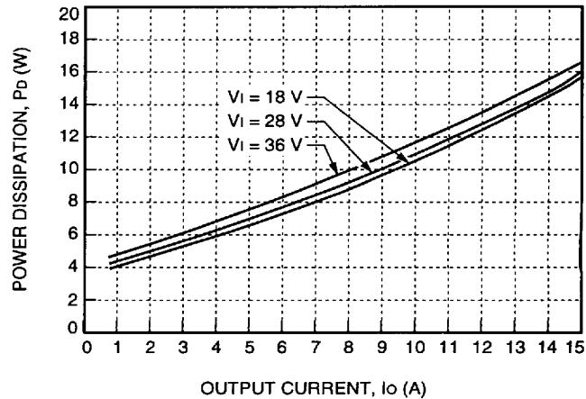
Figure 26. JC075A Power Dissipation vs. Output Current
