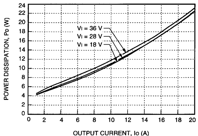
Figure 27. JC100A Power Dissipation vs. Output Current
