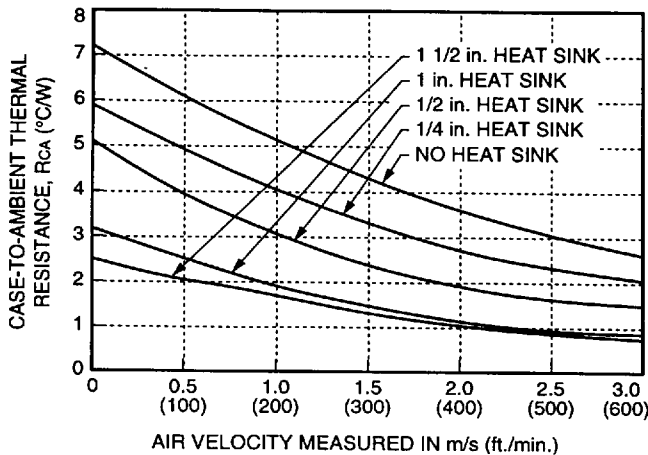
Figure 28. Case-to-Ambient Thermal Resistance Curves; Either Orientation
