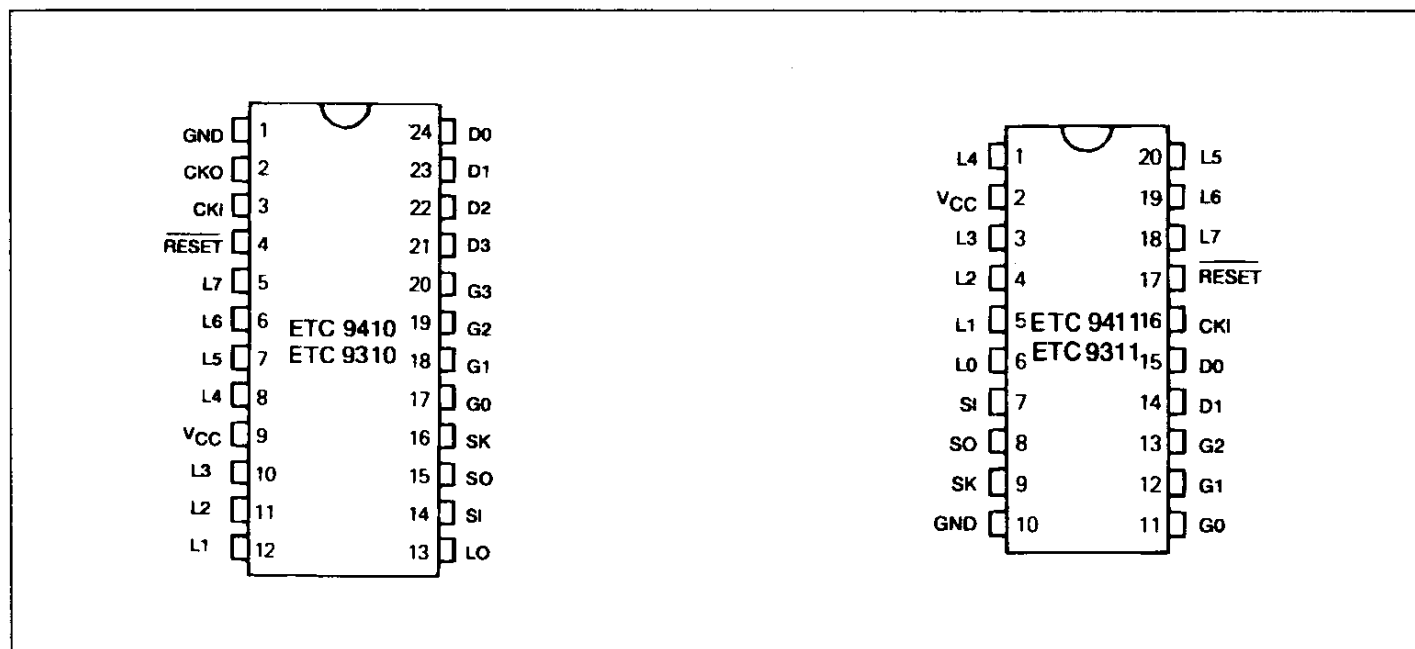
Figure 2 : Pin Connections.
