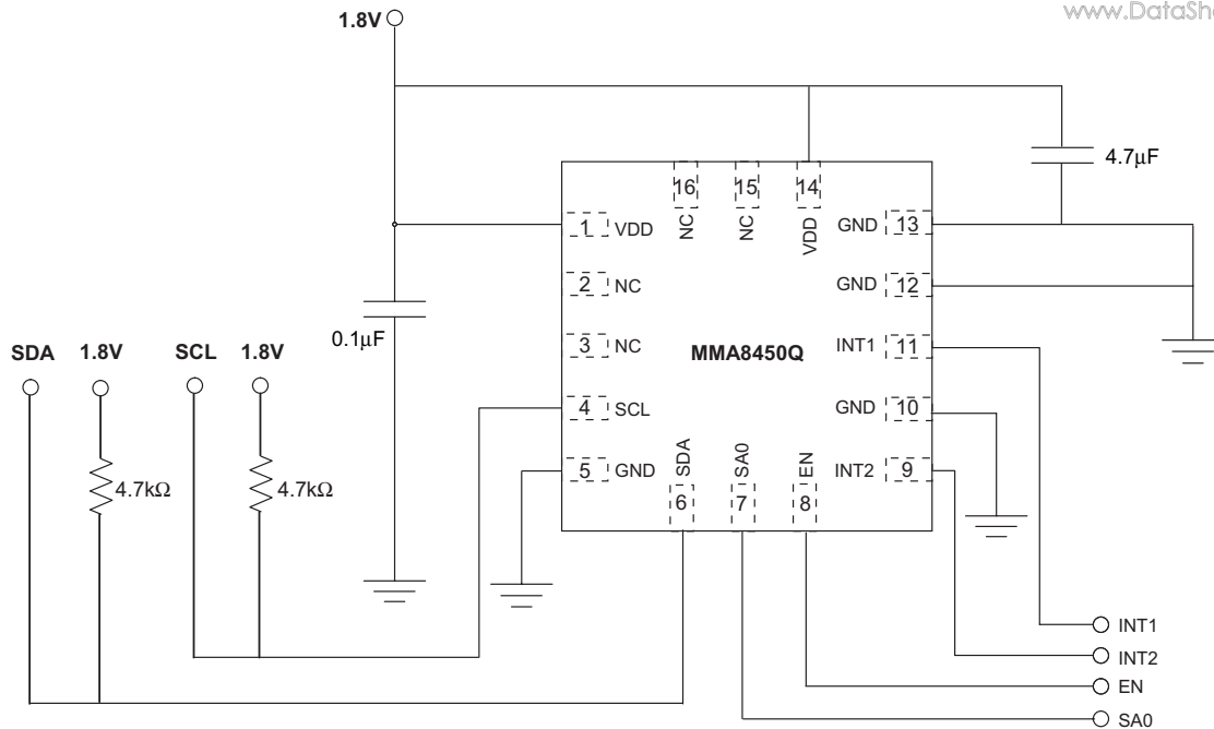
Figure 3. Application Diagram
