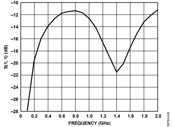
Figure 49. Differential RF Port Return Loss
