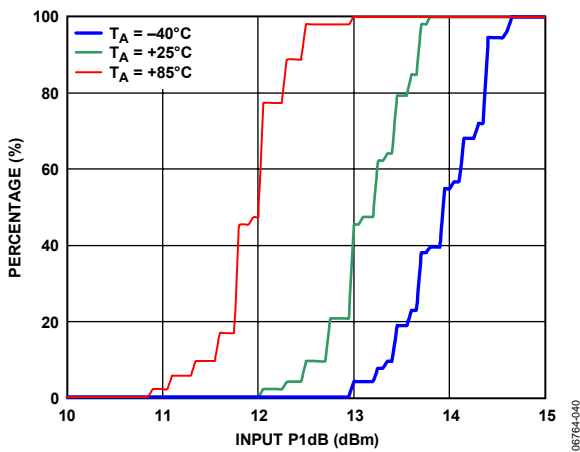
Figure 40. IP1dB Distributions
