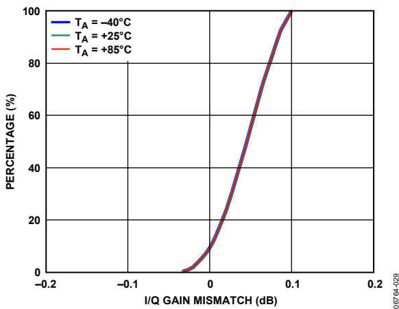
Figure 29. I/Q Gain Mismatch Distributions
