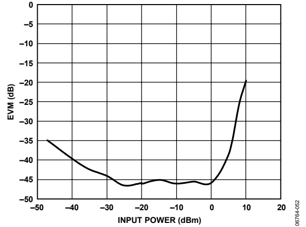
Figure 52. RF = 750MHz MHz, IF = 0 Hz, EVM vs. Input Power for a 16 QAM 10 MHz Bandwidth Mobile WiMAX Signal (AC-Coupled Baseband Outputs)
