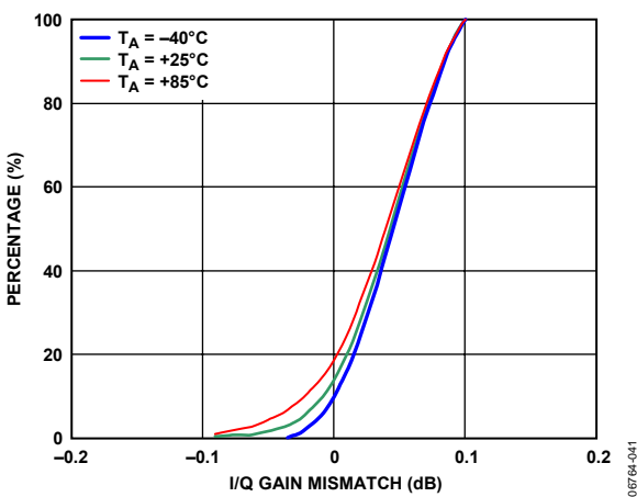
Figure 41. I/Q Gain Mismatch Distributions
