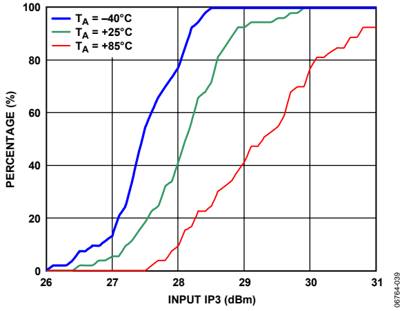
Figure 39. IIP3 Distributions
