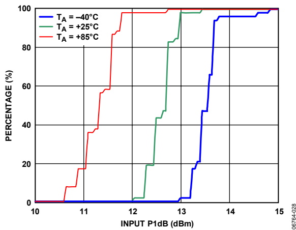
Figure 28. IP1dB Distributions
