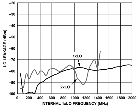
Figure 18. LO-to-RF Leakage vs. Internal 1xLO Frequency
