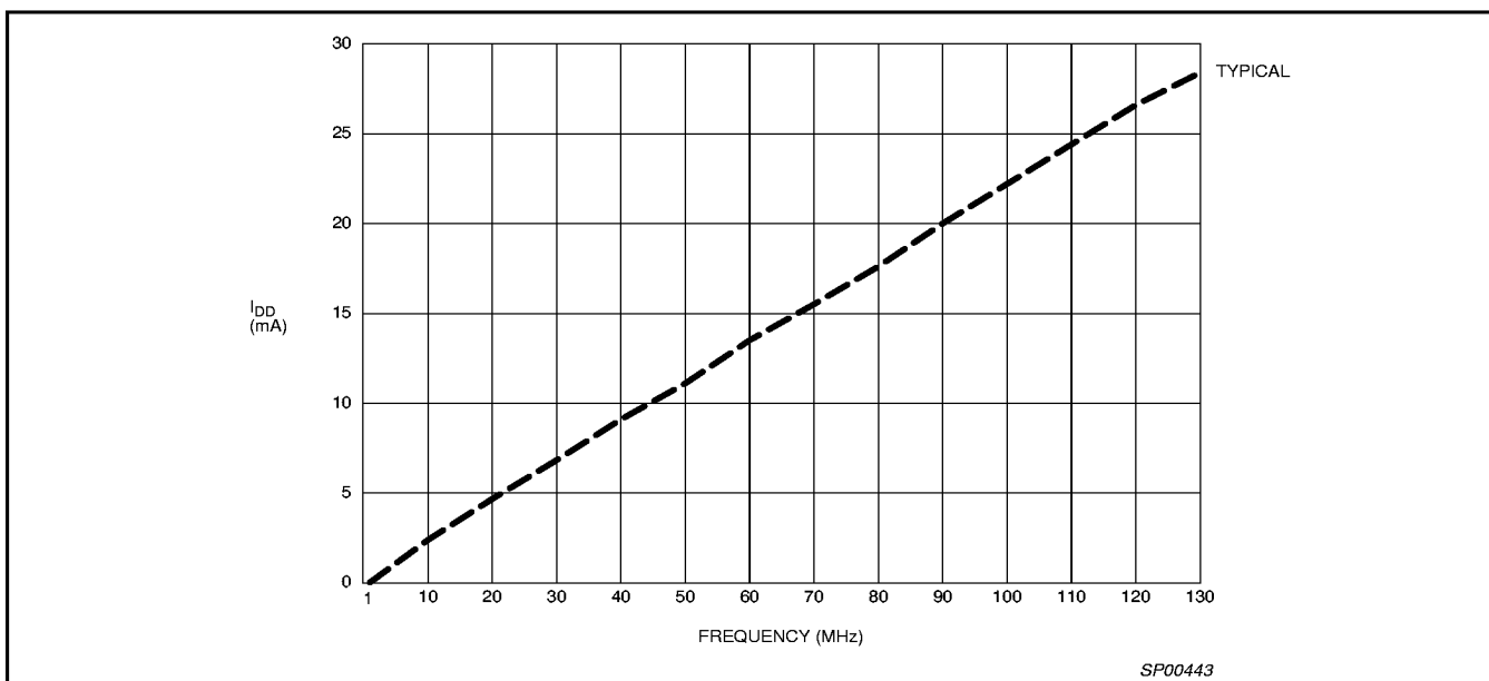
Figure 5. I DD vs. Frequency @ V DD = 3.3V
