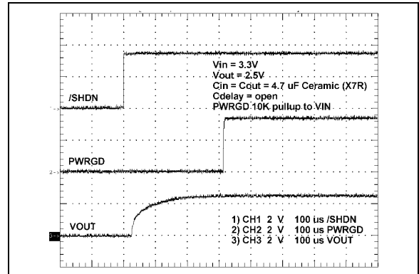
FIGURE 2-28: 2.5V (Fixed) Startup from Shutdown.
