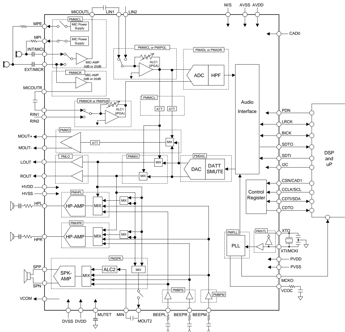
Figure 1. Block Diagram
