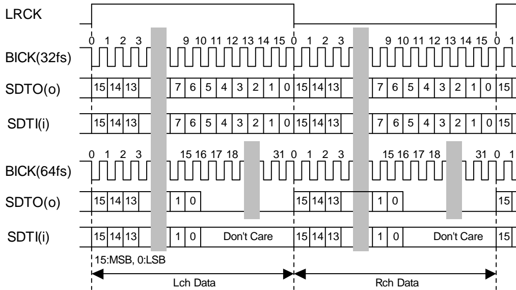
Figure 17. Mode 1 Timing
