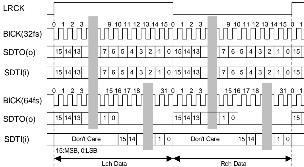
Figure 16. Mode 0 Timing
