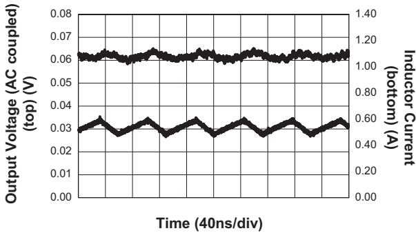
Output Ripple ( V_{IN} = 3.6V ; V_{OUT} = 1.8V ; Load = 3Ω)
