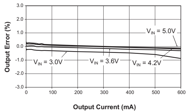
DC Regulation ( V_{OUT} = 2.5V ; L = 6.8\mu H )
