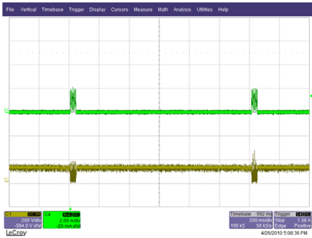
Figure 25 – 90 VAC, Full Load. Upper: I_{OUTPUT} , 2 A / div. Lower: V_{DRAIN} , 200 V, 200 ms / div.
