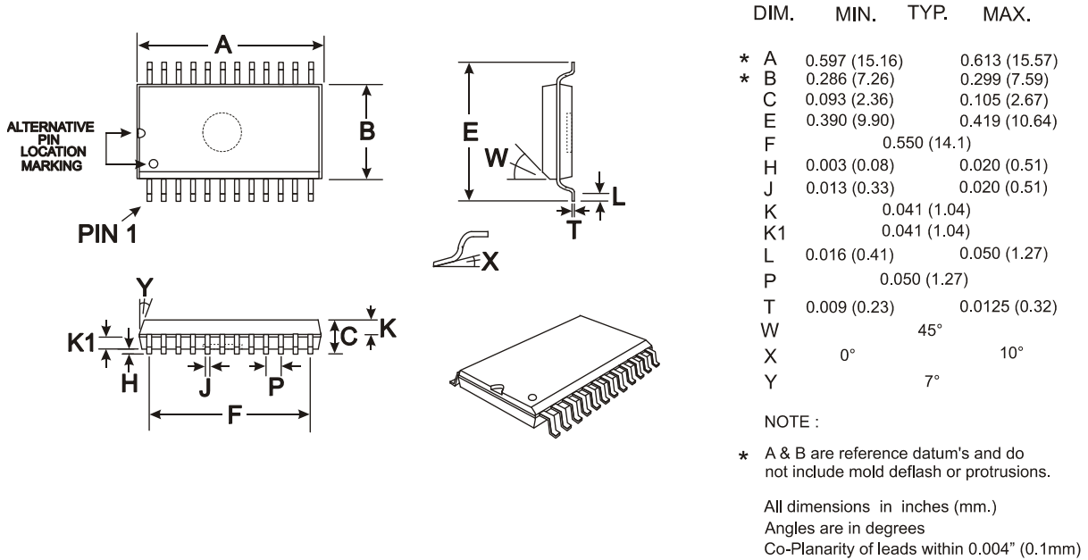
Figure 5 Mechanical Outline: Order as part no. FX828D2
