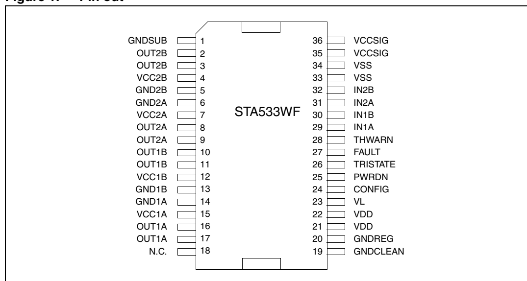
Figure 1. Pin out
