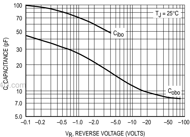
Figure 5. MPSA55/56 Capacitance
