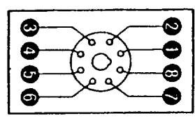
Terminal Arrangement (Top View)
