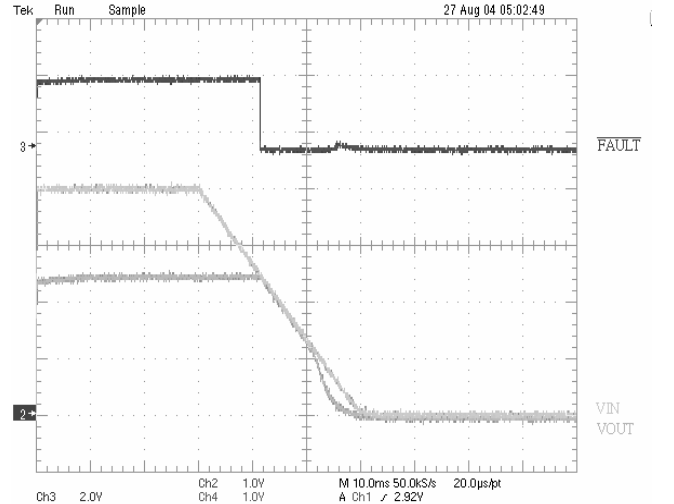
Power-down Response
