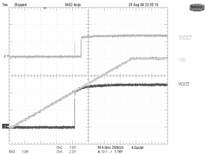
Power-up Response
