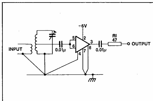
Fig. 7 RF preamplifier
