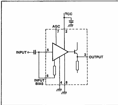
Fig. 2 Block diagram
