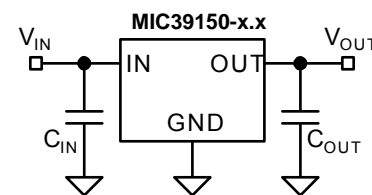
Figure 1. Capacitor Requirements
