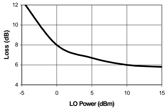
Conversion Loss vs. LO Power (LO = 200 MHz, RF = 140 MHz @ -10 dBm, IF = 60 MHz)
