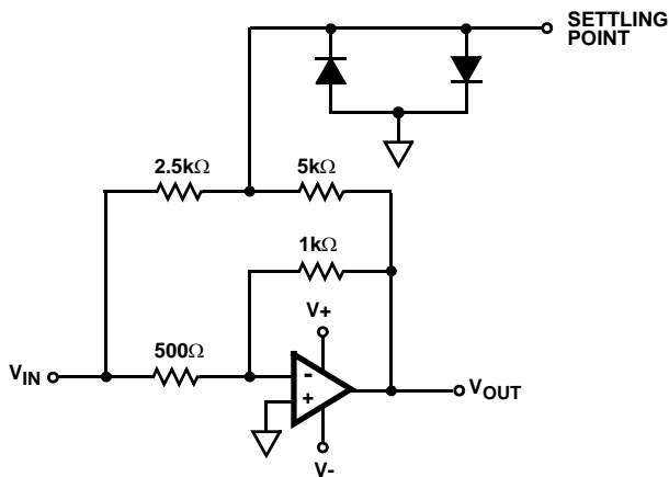
SETTLING TIME TEST CIRCUIT
