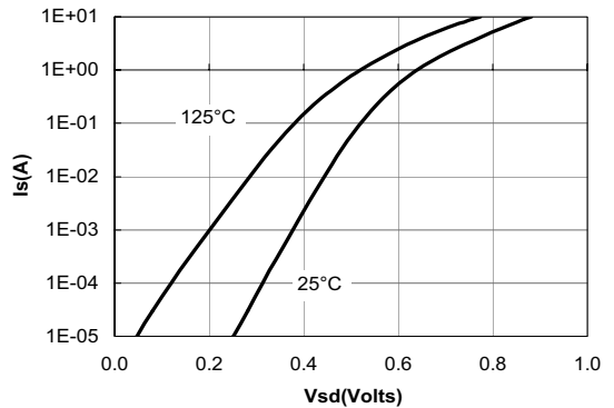
Figure 6: Body-Diode Characteristics
