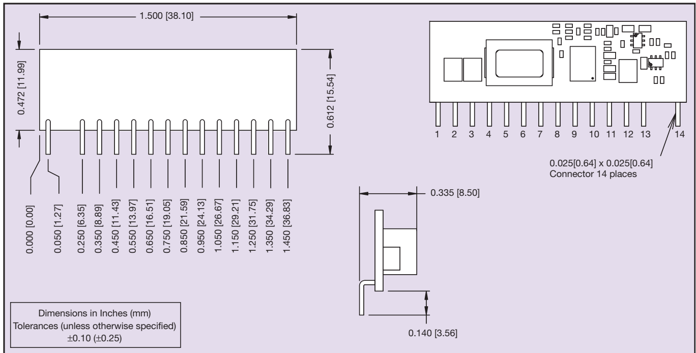
Figure 6 - Mechanical Drawing
