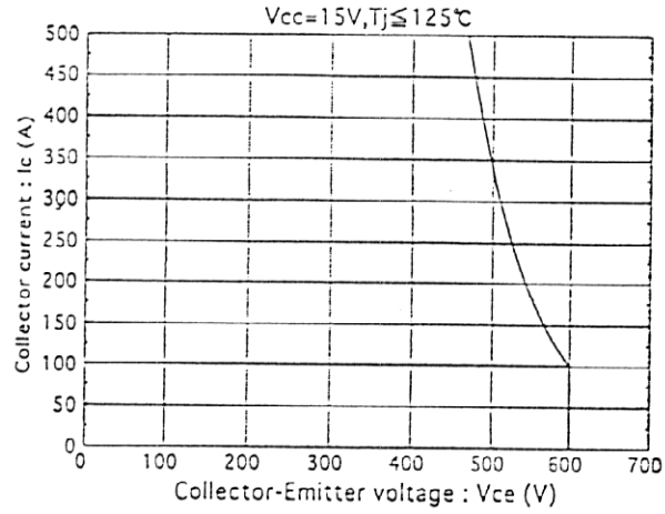
Reversed biased safe operating area
