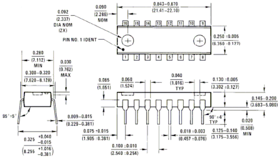
Molded Dual-In-Line Package (N)
