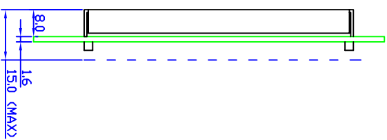
DETAIL FOR DOTS SCALE 16:1
