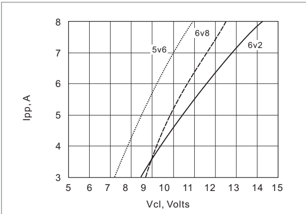
Clamping Voltage vs Ipp 8x20µsec Surge
