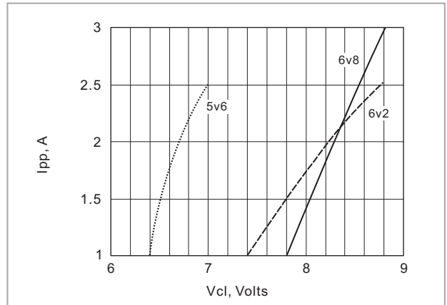
Clamping Voltage vs 10x1000µsec
