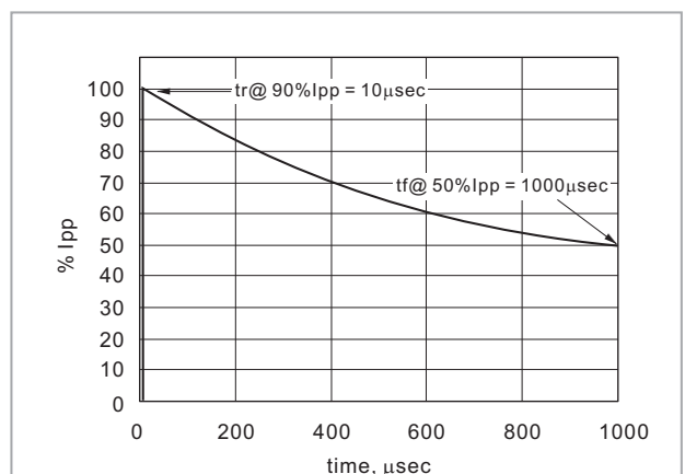
10x1000µsec Waveform
