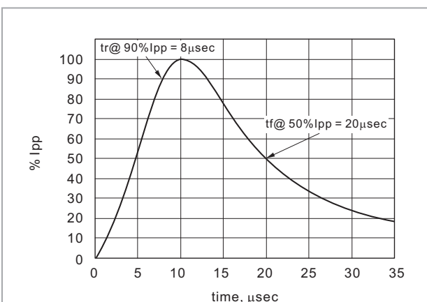
8x20µsec Surge Waveform
