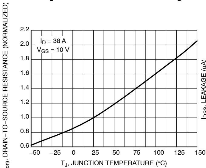
Figure 5. On-Resistance Variation with Temperature
